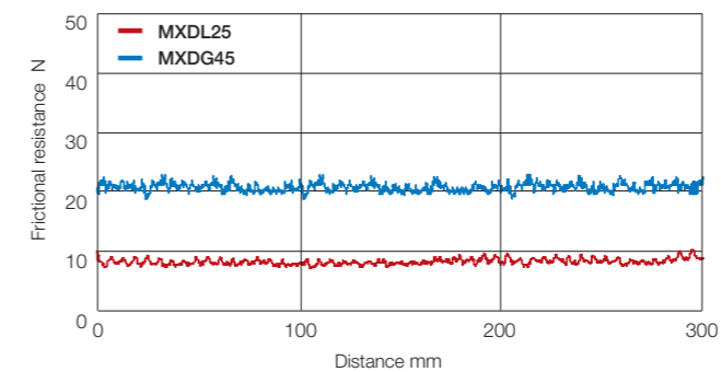
MXDL25 and MXDG45 T 3 preload frictional resistance
